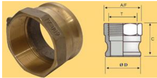
Camlock女性适配器阿
